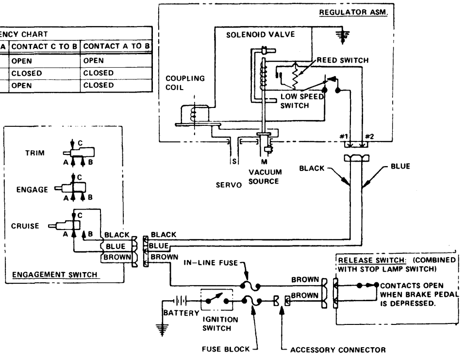
PONTIAC CRUISE CONTROL WIRING
