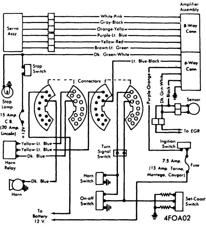
FORD MOTOR CO. SPEED CONTROL WIRING (EXC. MARK IV & THUNDERBIRD)
