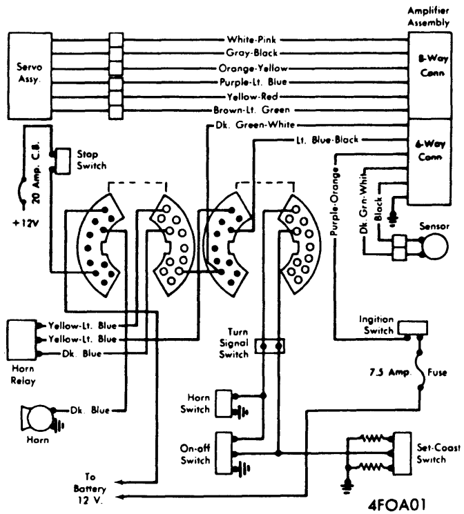
FORD MOTOR CO. SPEED CONTROL WIRING (MARK IV & THUNDERBIRD)
