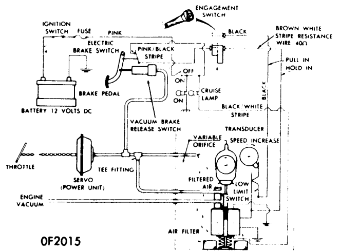
CHRYSLER CORP. SPEED CONTROL WIRING
