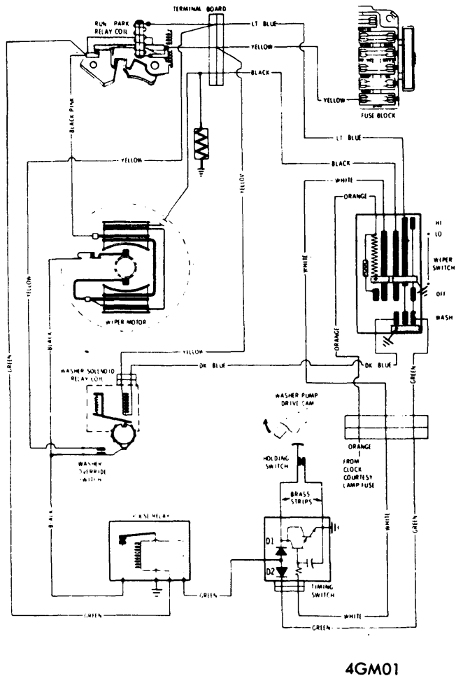
PULSE WIPER WIRING DIAGRAM (OLDSMOBILE)
