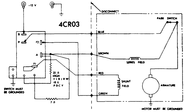
CHRYSLER CORP. THREE SPEED WIPER SYSTEM WIRING DIAGRAM
