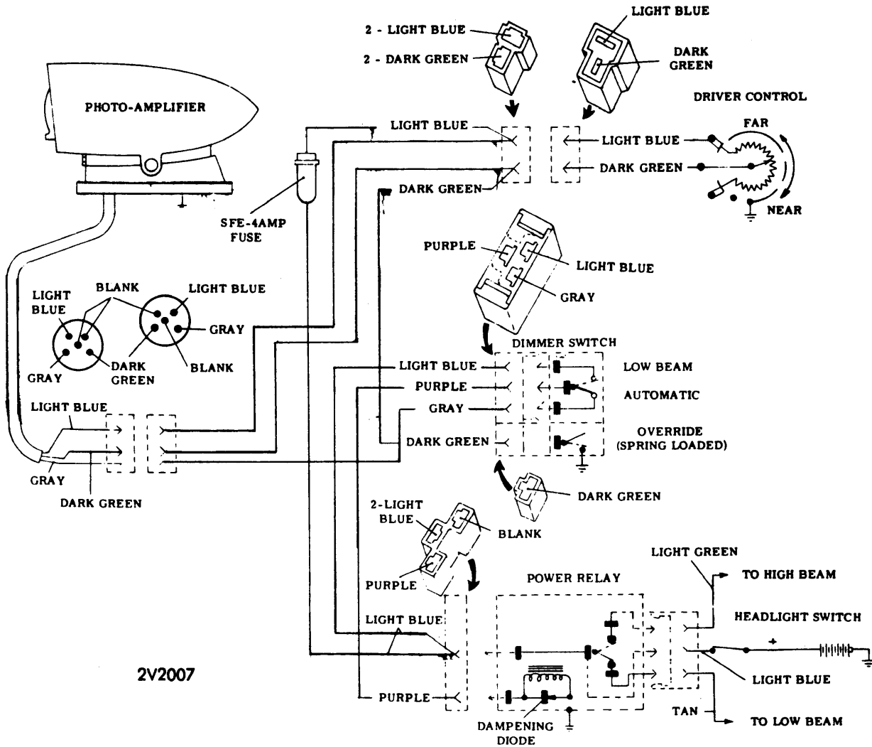
BUICK GUIDE-MATIC WIRING
