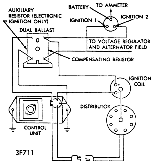
CHRYSLER CORP. ELECTRONIC IGNITION SYSTEM WIRING
