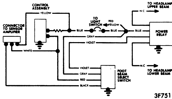
FORD MOTOR CO. HEADLIGHT DIMMER WIRING
