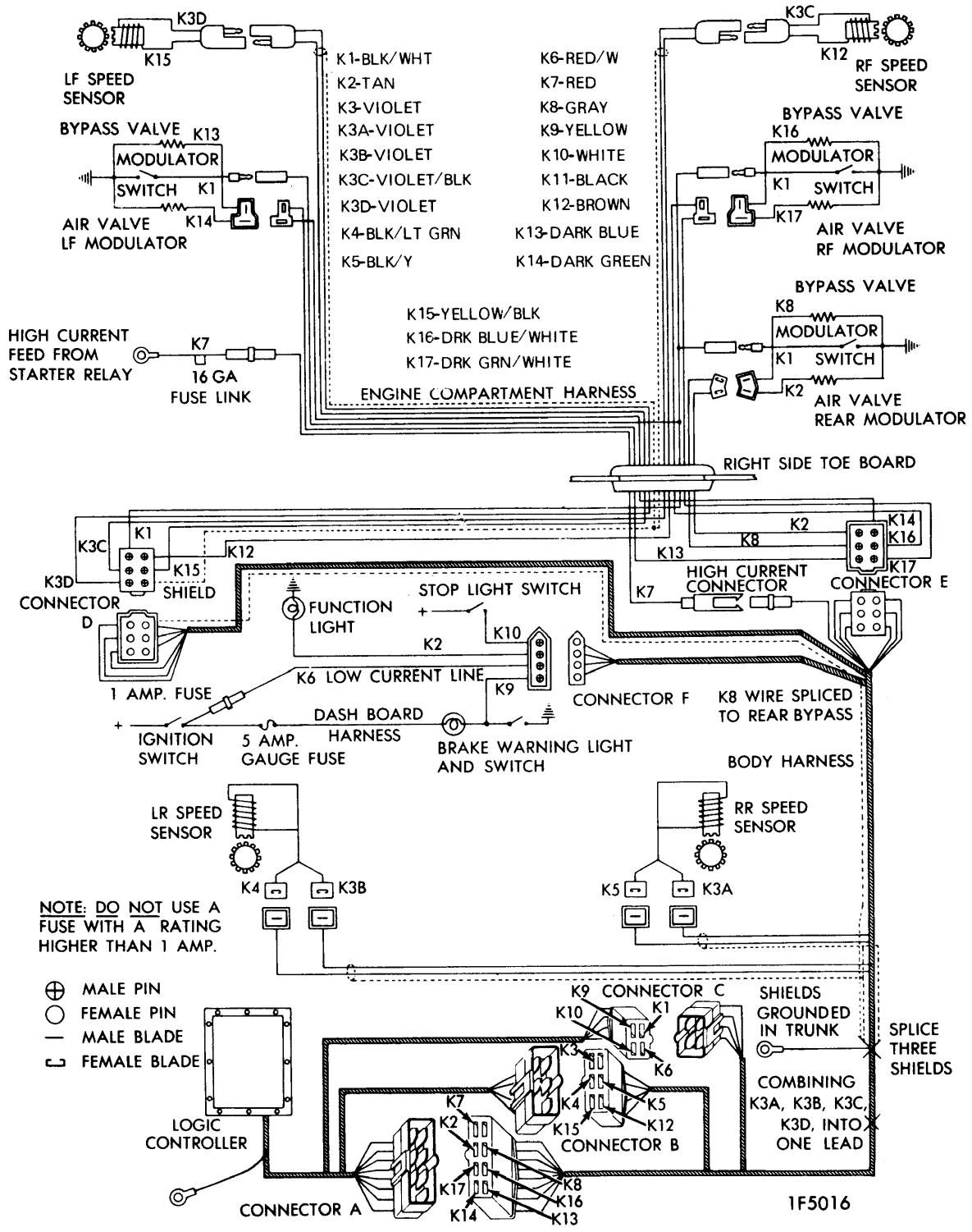
CHRYSLER CORP. SURE BRAKE WIRING
