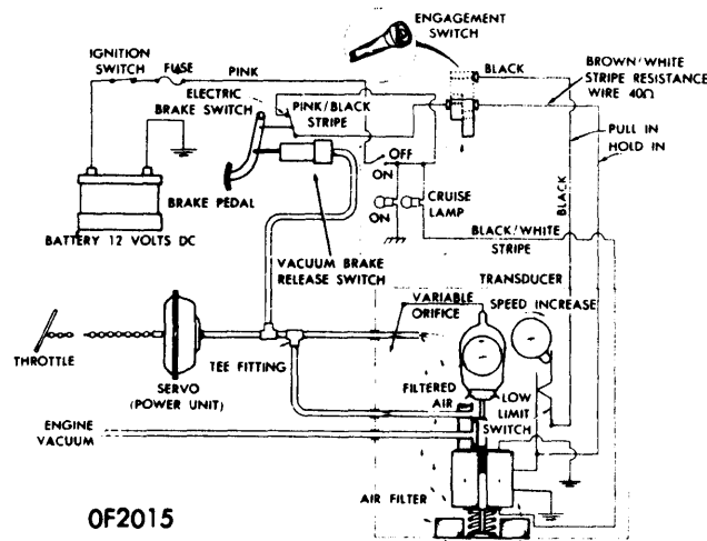
CADILLAC VACUUM & ELECTRICAL SPEED CONTROL SYSTEM
