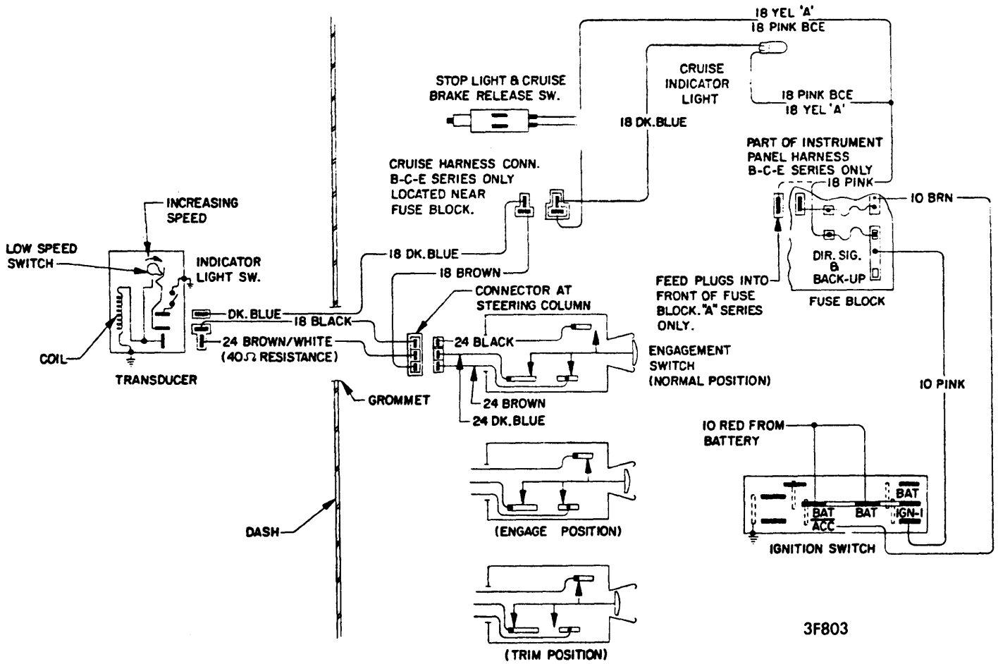
BUICK CRUISE MASTER WIRING
