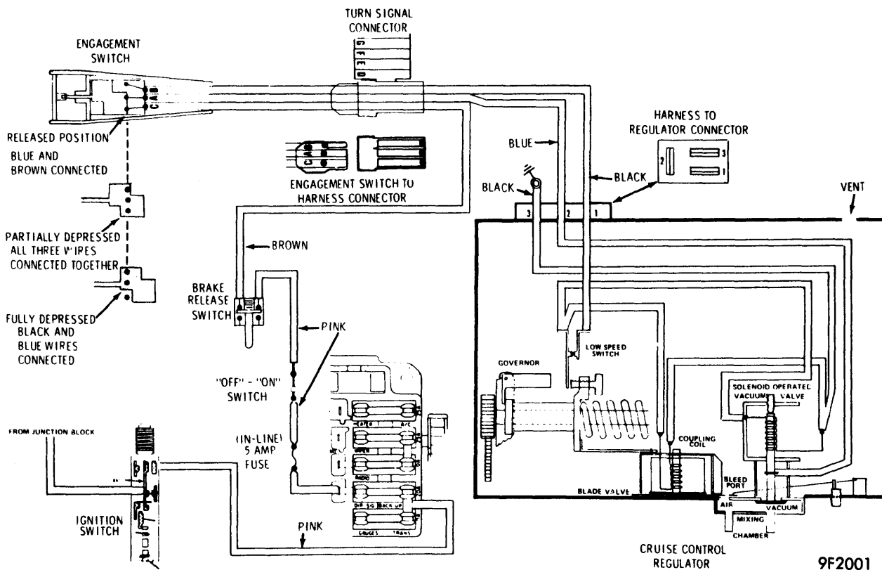
OLDSMOBILE SPEED CONTROL WIRING (PONTIAC SIMILAR)
