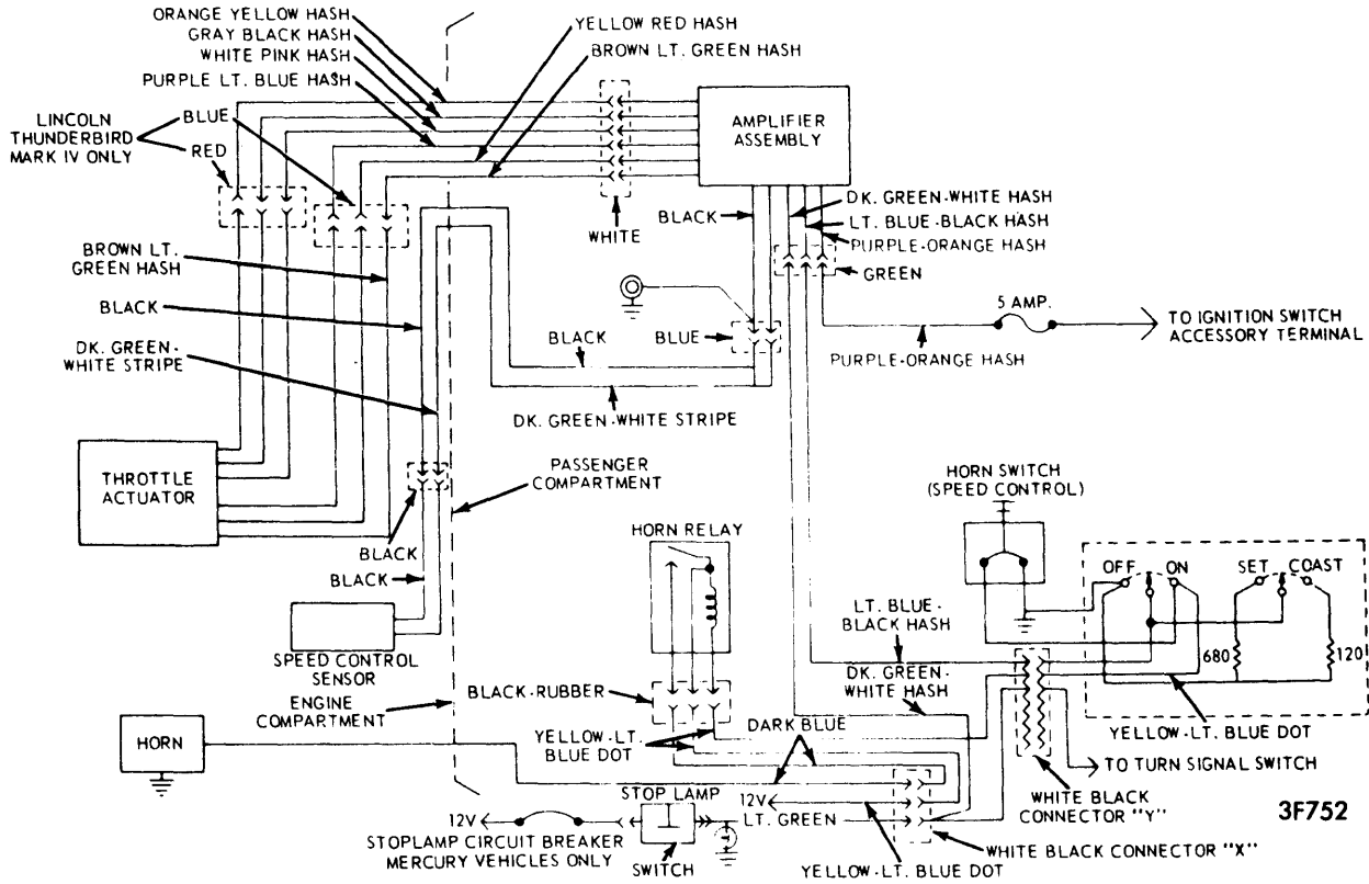
FORD MOTOR CO. SPEED CONTROL WIRING
