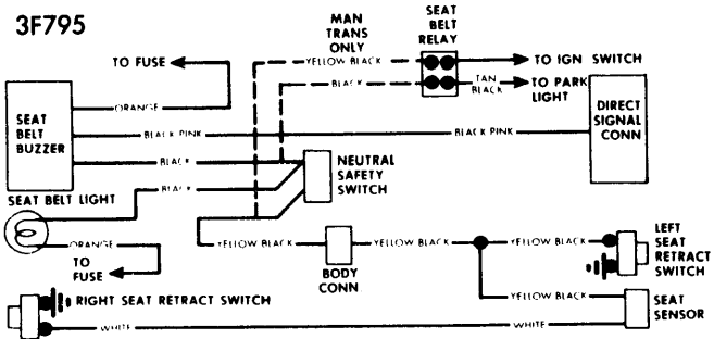
CHEVELLE & MONTE CARLO SEAT BELT WARNING SYSTEM
