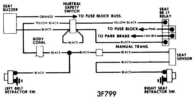
VENTURA & NOVA SEAT BELT WARNING SYSTEM
