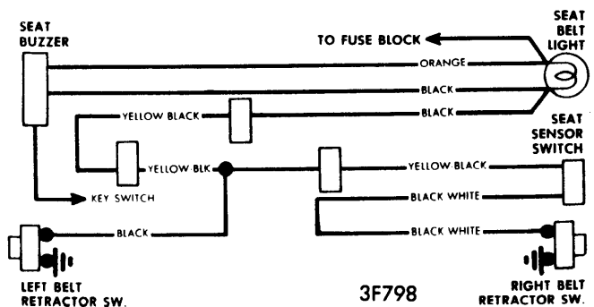
OMEGA SEAT BELT WARNING SYSTEM
