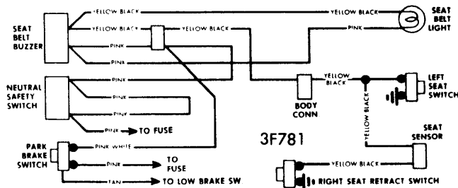
VEGA SEAT BELT WARNING SYSTEM
