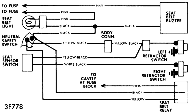
BUICK WITH MAN. TRANS. SEAT BELT WARNING SYSTEM
