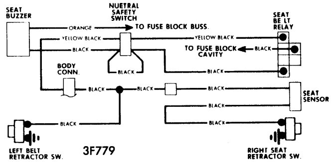
APOLLO WITH AUTO. TRANS. SEAT BELT WARNING SYSTEM
