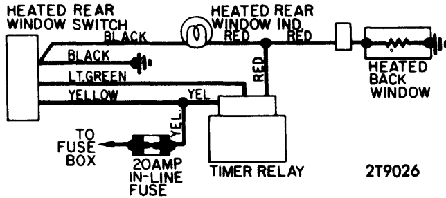
CADILLAC WINDOW DEFOGGER SYSTEM
