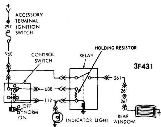
LINCOLN LATCHING RELAY WINDOW DEFOGGER SYSTEM
