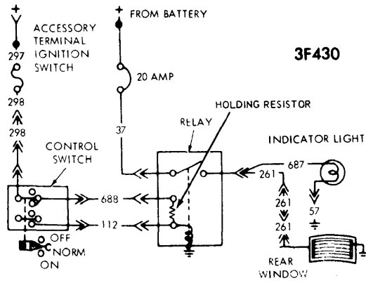
FORD MOTOR CO. (EXC. LINCOLN, MONTEGO, TORINO) LATCHING RELAY WINDOW DEFOGGER SYSTEM
