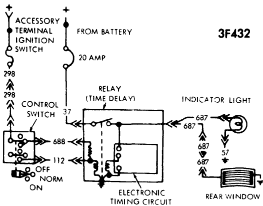
MONTEGO & TORINO TIME DELAY WINDOW DEFOGGER SYSTEM
