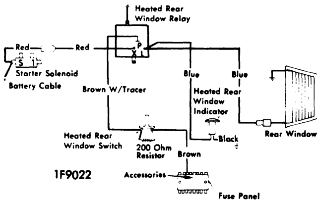
AMERICAN MOTORS (JAVELIN) WINDOW DEFOGGER SYSTEM
