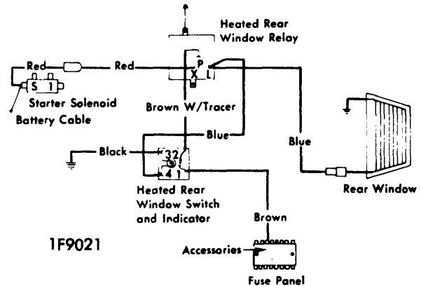
AMERICAN MOTORS (MATADOR, AMBASSADOR) WINDOW DEFOGGER SYSTEM
