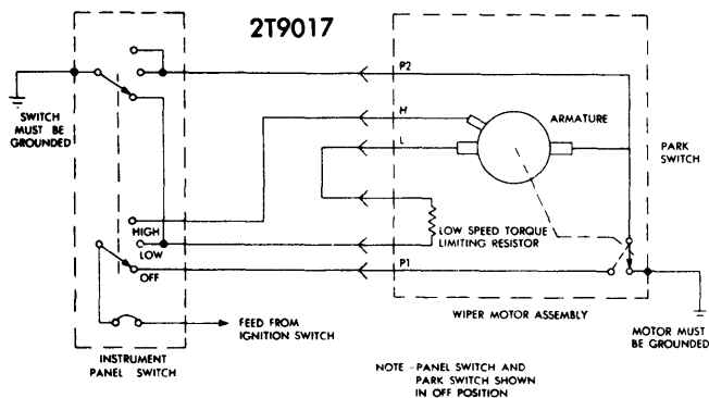
CHRYSLER CORP. 2-SPEED WIPER SYSTEM (CONCEALED WIPERS)
