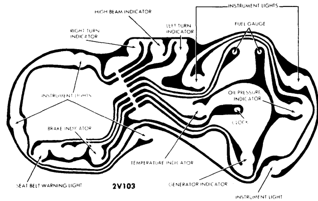
CATALINA, BONNEVILLE & GRAND VILLE (WITH INDICATOR LIGHTS)
