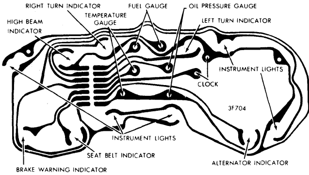
LEMANS, LEMANS SPORT, LUXURY LEMANS & GRAND AM (WITH GAUGES)
