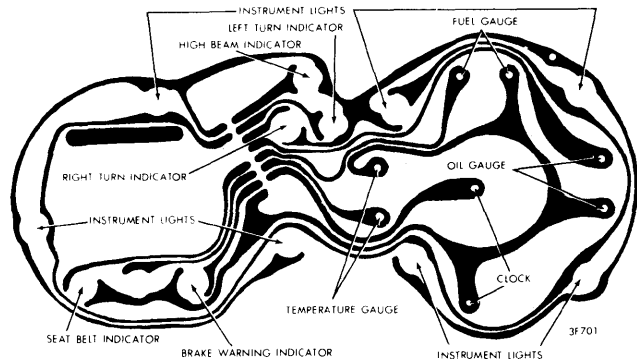
CATALINA, BONNEVILLE & GRAND VILLE (WITH GAUGES)
