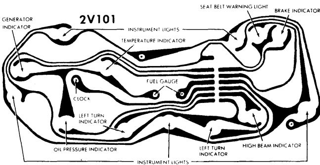
FIREBIRD (WITH INDICATOR LIGHTS)
