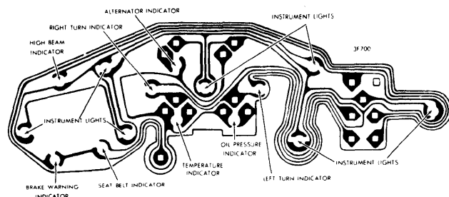
GRAND PRIX (WITH INDICATOR LIGHTS)
