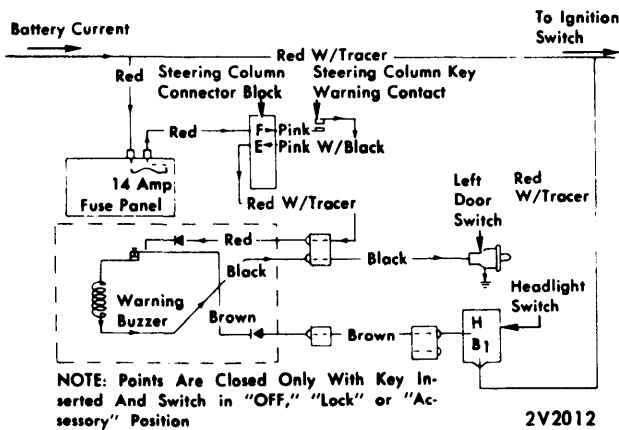
AMERICAN MOTORS BUZZER WIRING DIAGRAM
