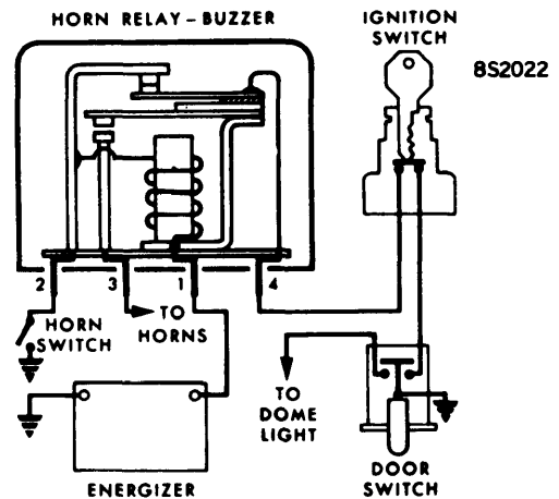
GM HORN RELAY-BUZZER WIRING DIAGRAM
