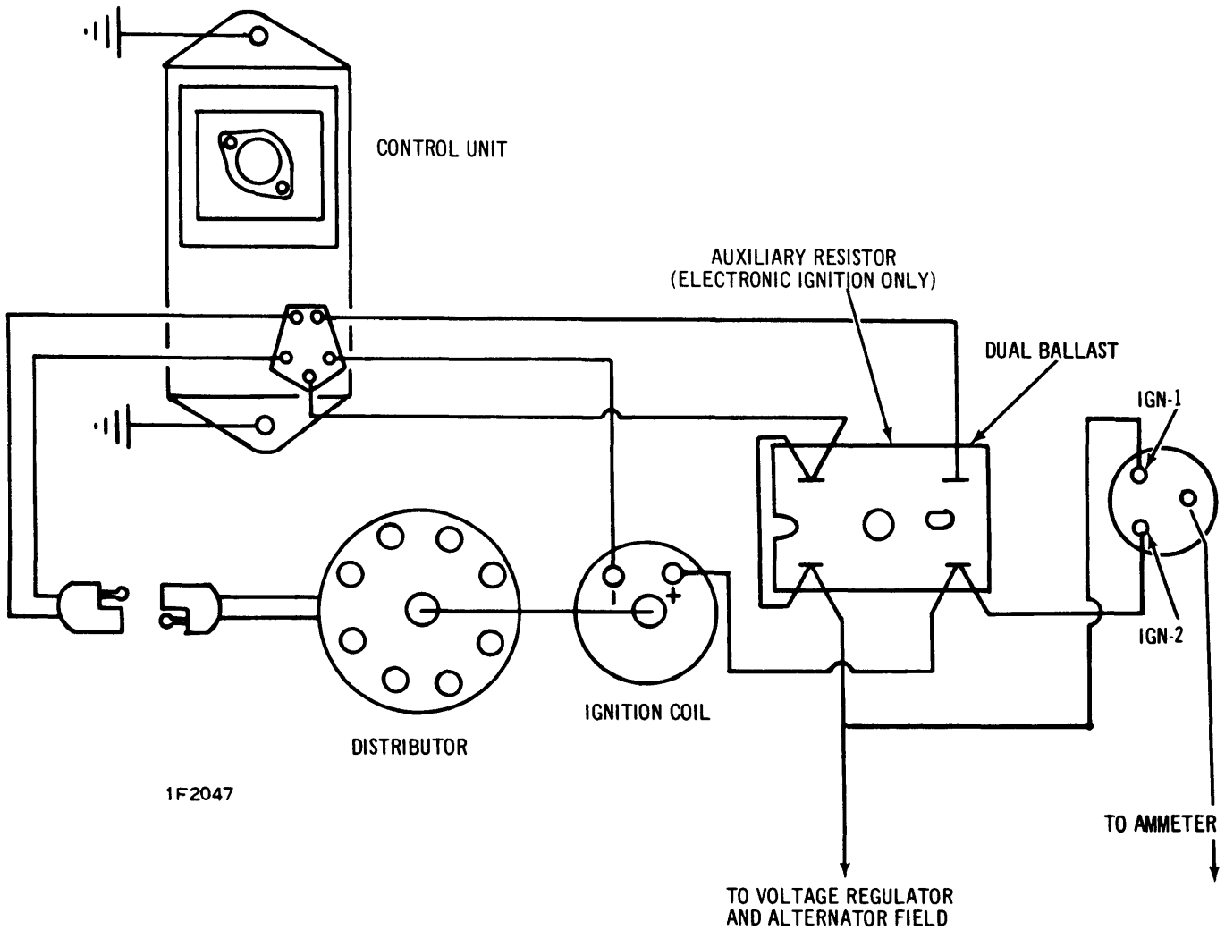
CHRYSLER CORP. ELECTRONIC IGNITION SYSTEM WIRING SCHEMATIC
