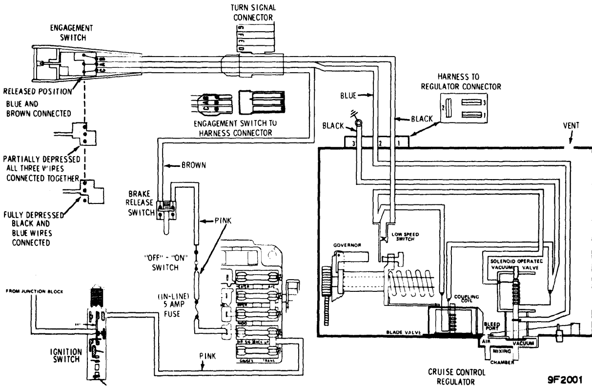
OLDSMOBILE CRUISE CONTROL ELECTRICAL CIRCUIT (PONTIAC SIMILAR)
