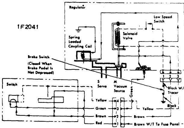
American Motors CRUISE COMMAND WIRING DIAGRAM
