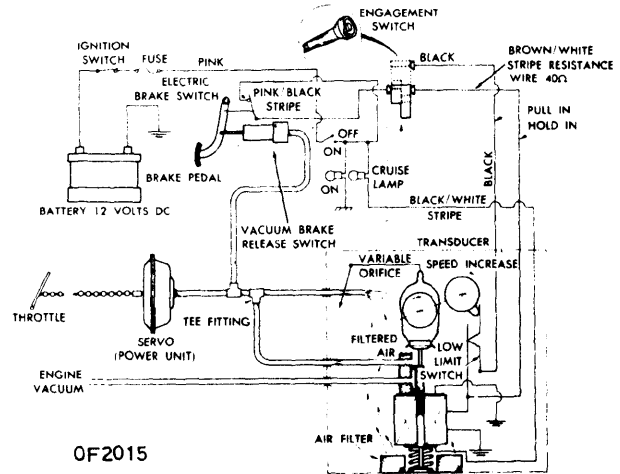
CADILLAC VACUUM & ELECTRICAL DIAGRAM (ALL OTHER MODELS SIMILAR)
