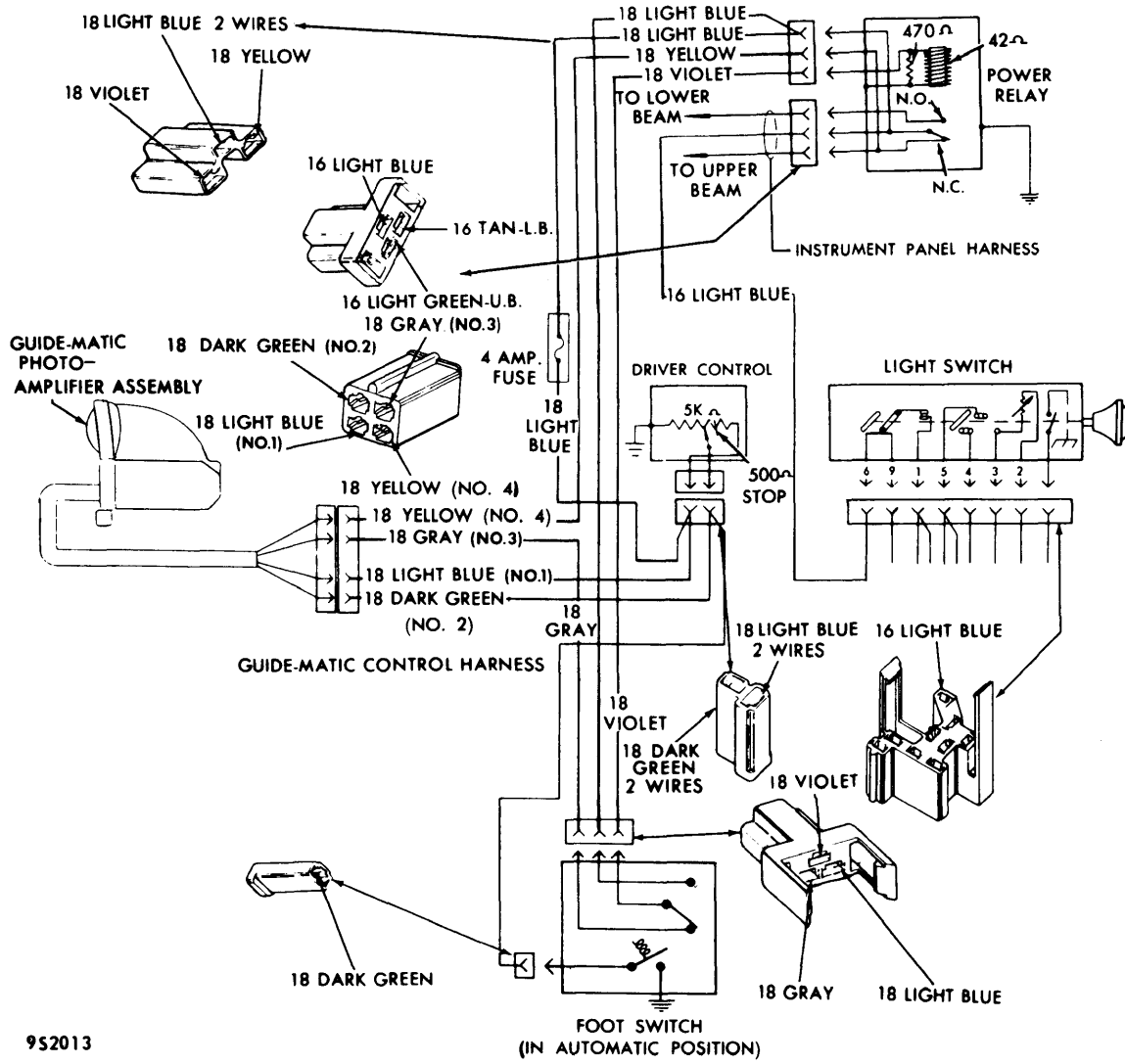
CADILLAC GUIDE-MATIC CIRCUIT DIAGRAM
