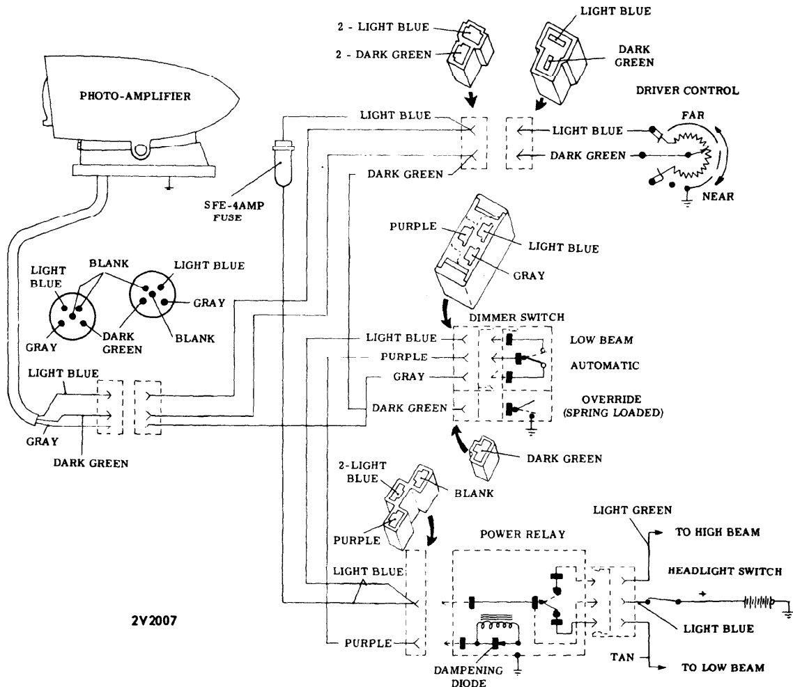
BUICK & OLDSMOBILE GUIDE-MATIC CIRCUIT DIAGRAM
