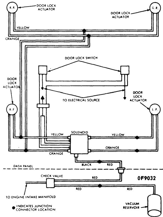
LINCOLN CONTINENTAL VACUUM/ELECTRIC DOOR LOCKS
