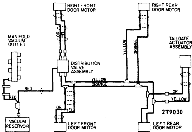
FORD, MERCURY, METEOR VACUUM DOOR LOCKS
