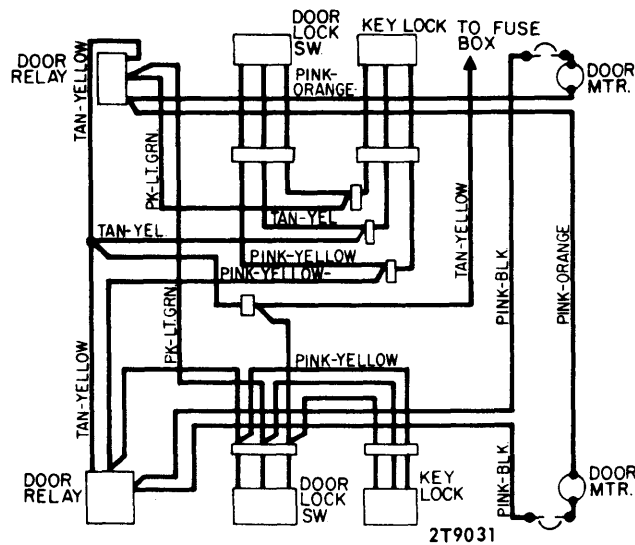
THUNDERBIRD, MARK IV ELECTRIC DOOR LOCKS
