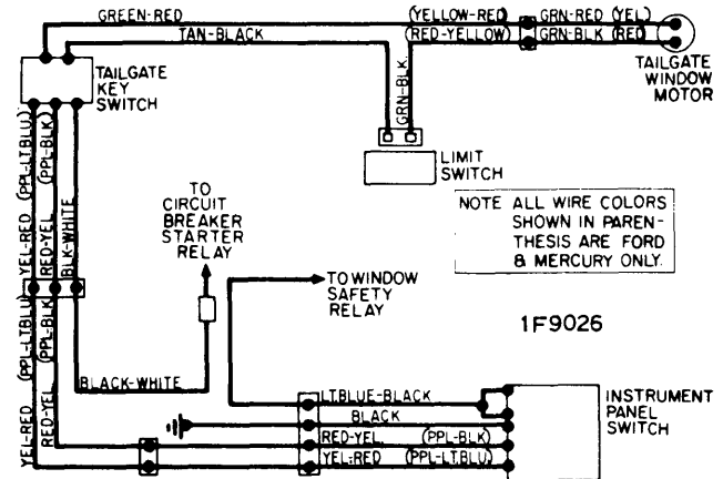
TAILGATE WINDOW WIRING DIAGRAM FORD, MERCURY, TORINO & MONTEGO
