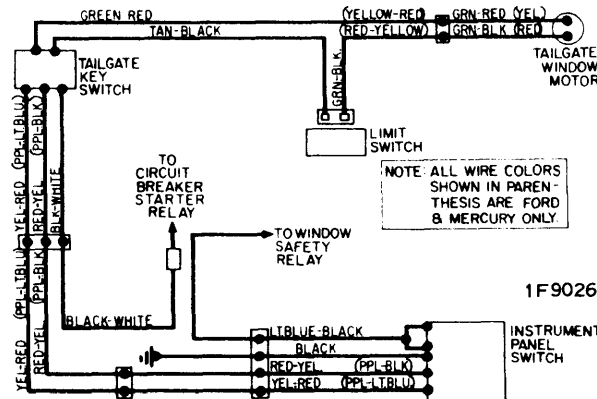
FORD MOTOR CO. TAILGATE POWER WINDOW
