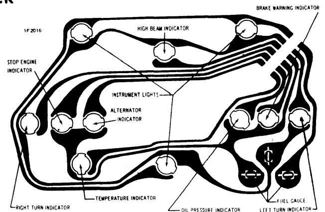
1972 BUICK LESABRE, ESTATE WAGON, CENTURION, ELECTRA & RIVIERA
