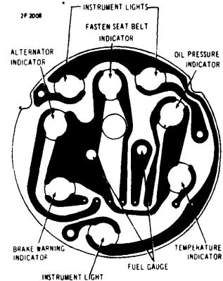
1972 F-85 (WITH INDICATOR LIGHTS)
