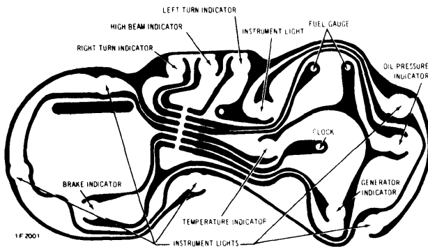
1972 CATALINA, BONNEVILLE & GRAND VILLE (WITH INDICATOR LIGHTS)
