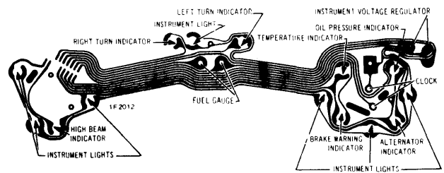
1972 MUSTANG WITHOUT TACHOMETER
