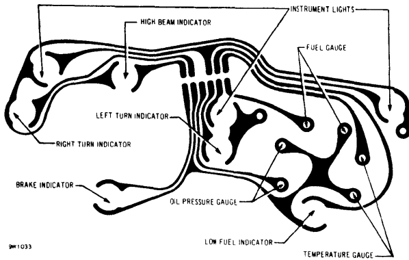
1972 LE MANS & GRAND PRIX (WITH GAUGES)
