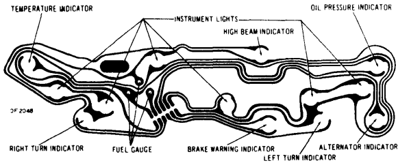
1972 CAMARO (WITH INDICATOR LIGHTS)
