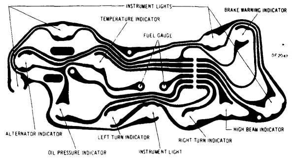
1972 FIREBIRD WITH INDICATOR LIGHTS
