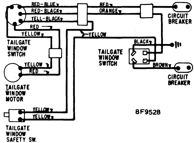
AMERICAN MOTORS TAILGATE WINDOW CONTROL WIRING DIAGRAM
