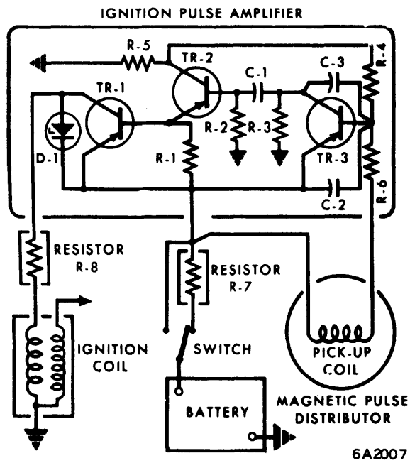
TRANSISTOR IGNITION AMPLIFIER CIRCUIT
