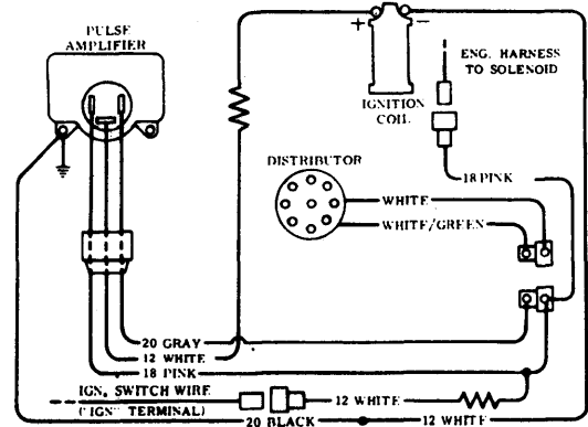
CORVETTE TRANSISTOR IGNITION CIRCUIT
