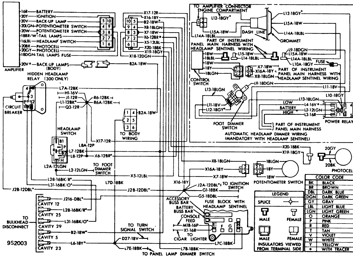
SAFEGUARD SENTINEL WIRING DIAGRAM
