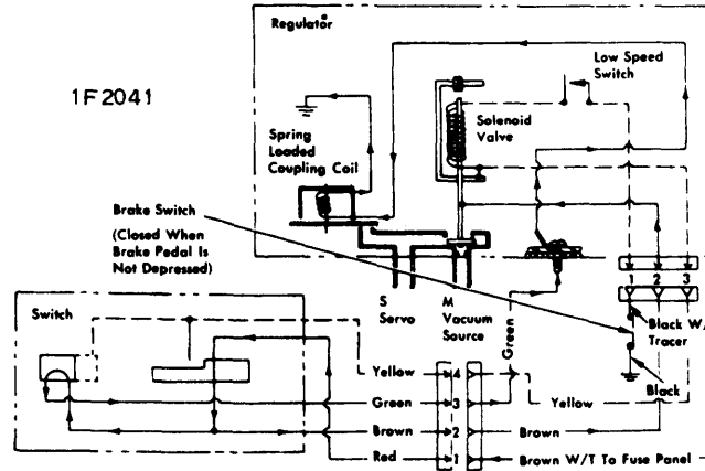
American Motors CRUISE COMMAND WIRING DIAGRAM
