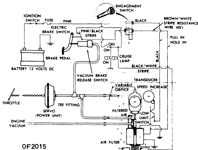
American Motors CRUISE COMMAND WIRING DIAGRAM
