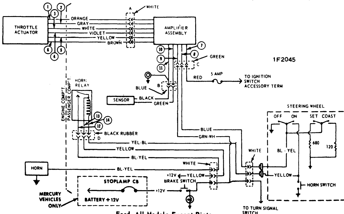
Ford, All Models Except Pinto Mercury, All Models Except Cougar Thunderbird SPEED CONTROL WIRING DIAGRAM
