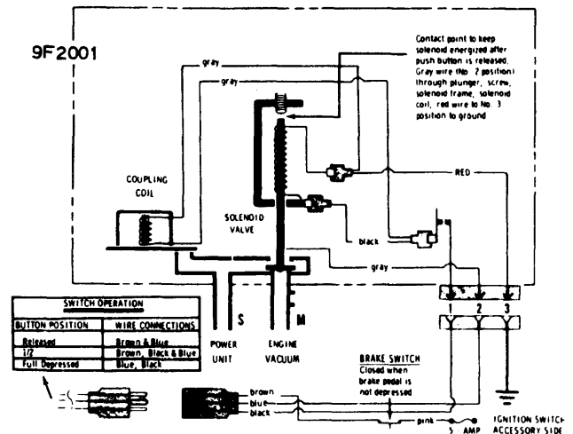
OLDSMOBILE CRUISE CONTROL ELECTRICAL CIRCUIT (PONTIAC SIMILAR)
