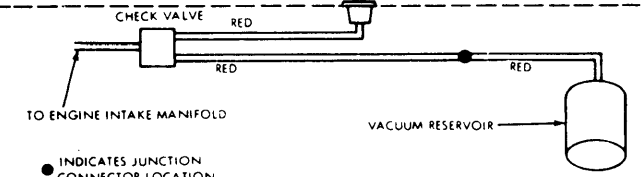
VACUUM DOOR LOCK SCHEMATIC (FORD, MERCURY & METEOR) CF9030
