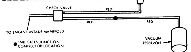
VACUUM DOOR LOCK SCHEMATIC (LINCOLN CONTINENTAL)
