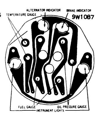
1971 F-85 (WITH GAUGES)
