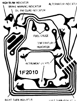
1971 OLDSMOBILE (EXCEPT F-85)
