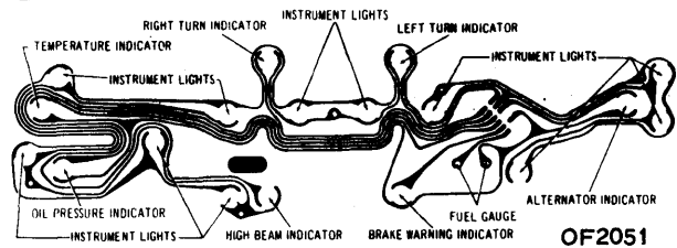
1971 CHEVELLE & MONTE CARLO (WITH INDICATOR LIGHTS)
