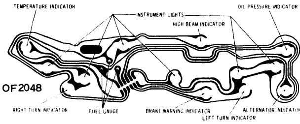
1971 CAMARO (WITH INDICATOR LIGHTS)
