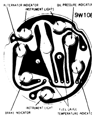
1971 F-85 (WITH INDICATOR LIGHTS)
