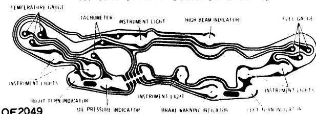
1971 CAMARO (WITH GAUGES)
