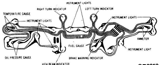
1971 CHEVELLE & MONTE CARLO (WITH GAUGES)
