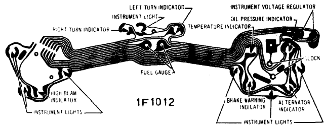
1971 MUSTANG WITHOUT TACHOMETER
