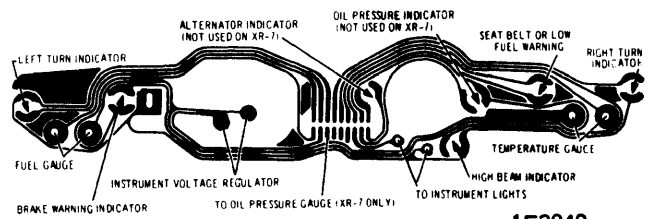
1971 COUGAR & COUGAR XR 7
