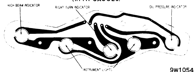
1971 DART (RIGHT SIDE)
