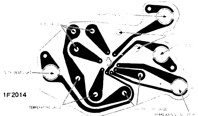
1971 VALIANT & DART (RIGHT SIDE) (WITH GAUGES)
