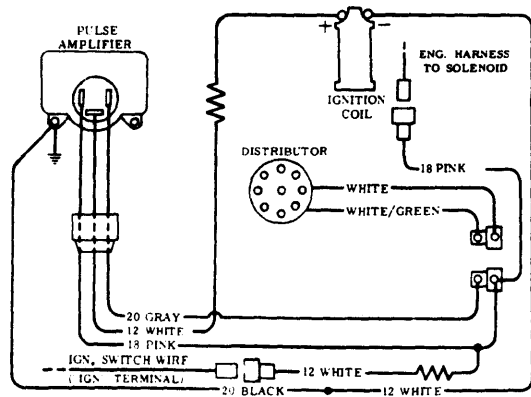
CORVETTE TRANSISTOR IGNITION CIRCUIT
