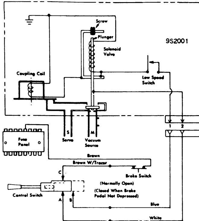
CRUISE COMMAND WIRING DIAGRAM
