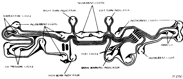
1970-72 CHEVELLE & 1971-72 MONTE CARLO (W/GAUGES)
