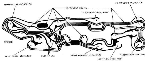
1970-72 CAMARO (W/INDICATOR LIGHTS)
