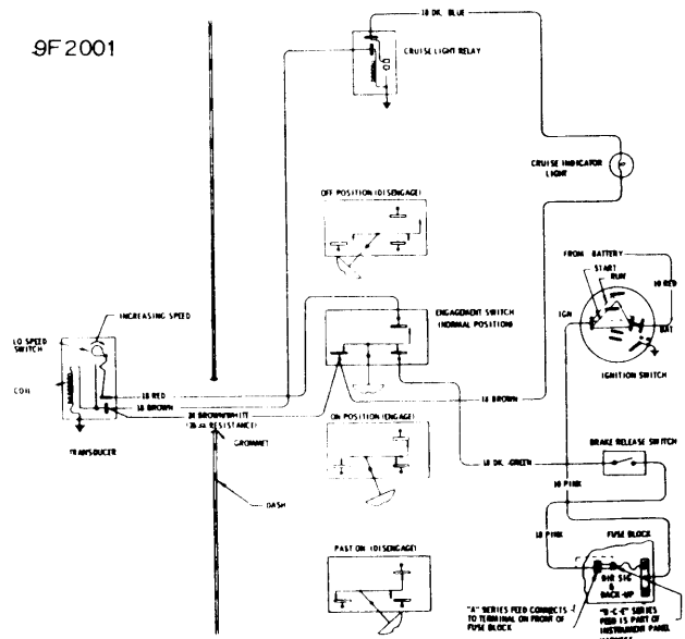
1969 GENERAL MOTORS CRUISE CONTROL (Exc. LESABRE, WILDCAT, ELECTRA & RIVIERA)
