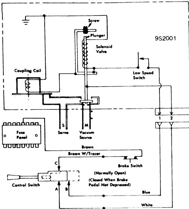
1969 AMERICAN MOTORS CRUISE COMMAND DIAGRAM
