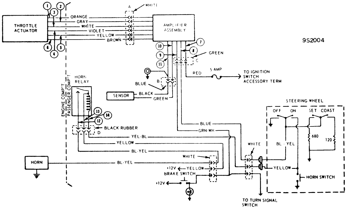
1969 FORD & MERCURY SPEED CONTROL DIAGRAM
