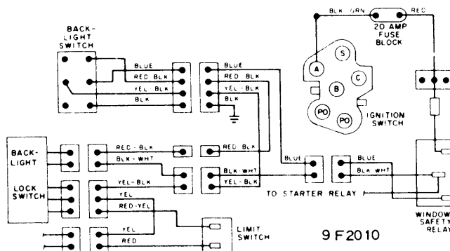
1969 FALCON, FAIRLANE & MONTEGO DUAL ACTION TAILGATE WIRING
