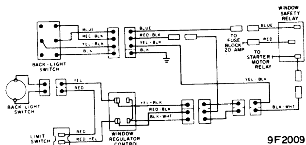
1969 FALCON, FAIRLANE & MONTEGO SINGLE ACTION TAILGATE WIRING
