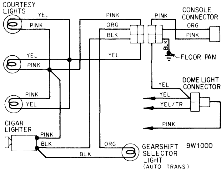
1969 CHRYSLER (EXC. IMPERIAL)
