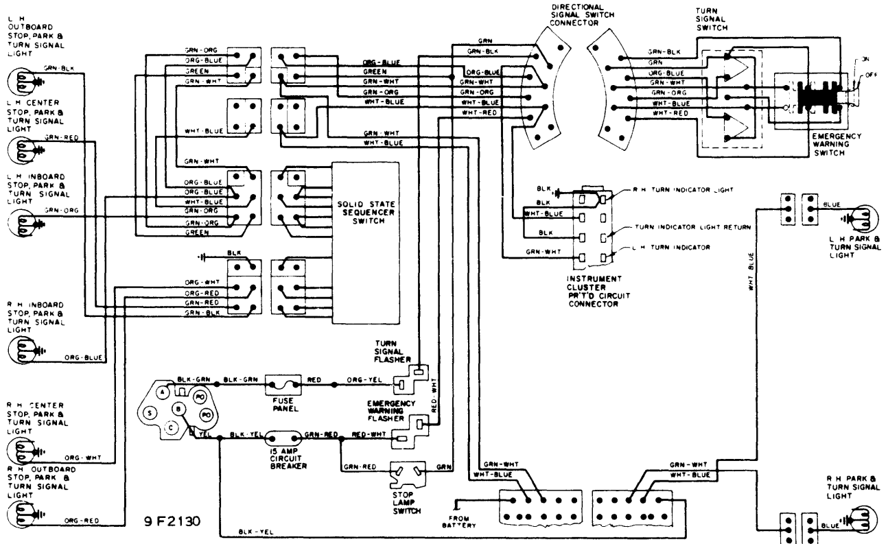
1969 THUNDERBIRD SEQUENTIAL DIRECTION SIGNALS (LATER TYPE-SOLID STATE FLASHER UNIT)
