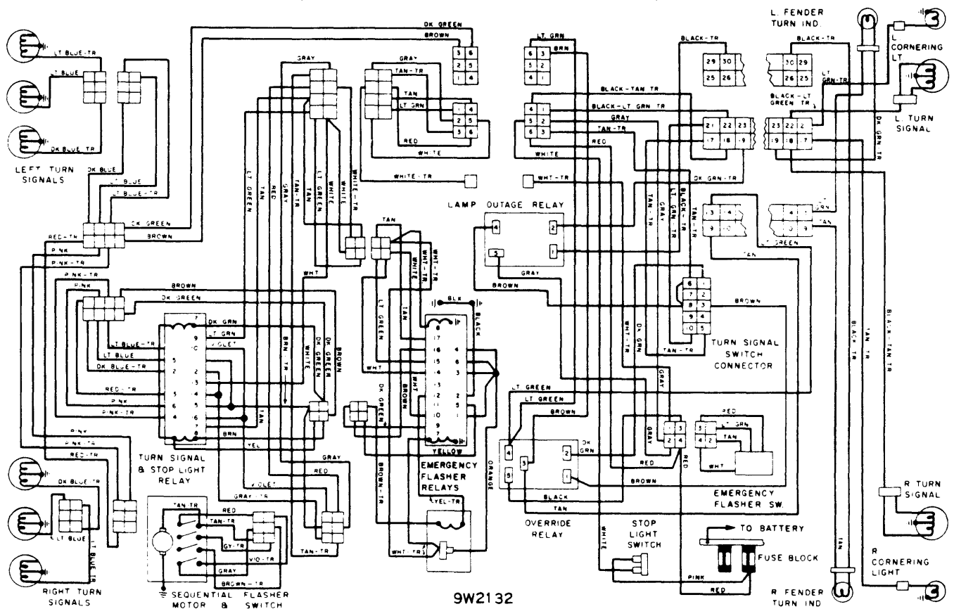
1969 CHRYSLER IMPERIAL SEQUENTIAL DIRECTION SIGNALS
