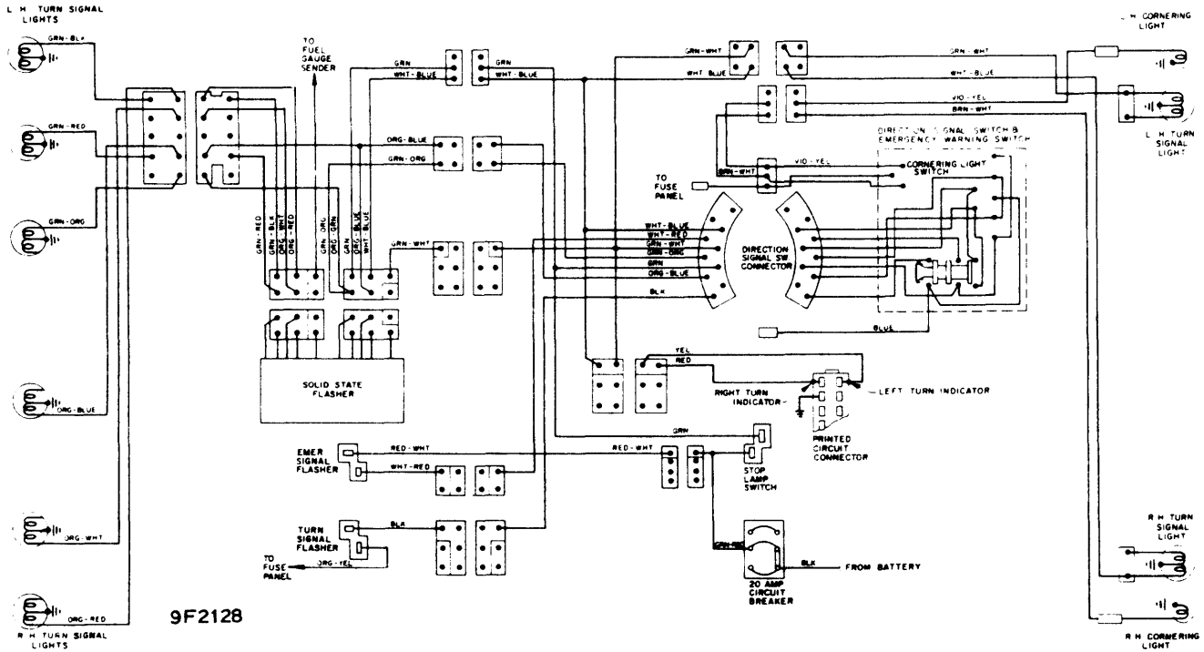
1969 COUGAR SEQUENTIAL DIRECTION SIGNALS (WITH SOLID STATE FLASHER UNIT)
