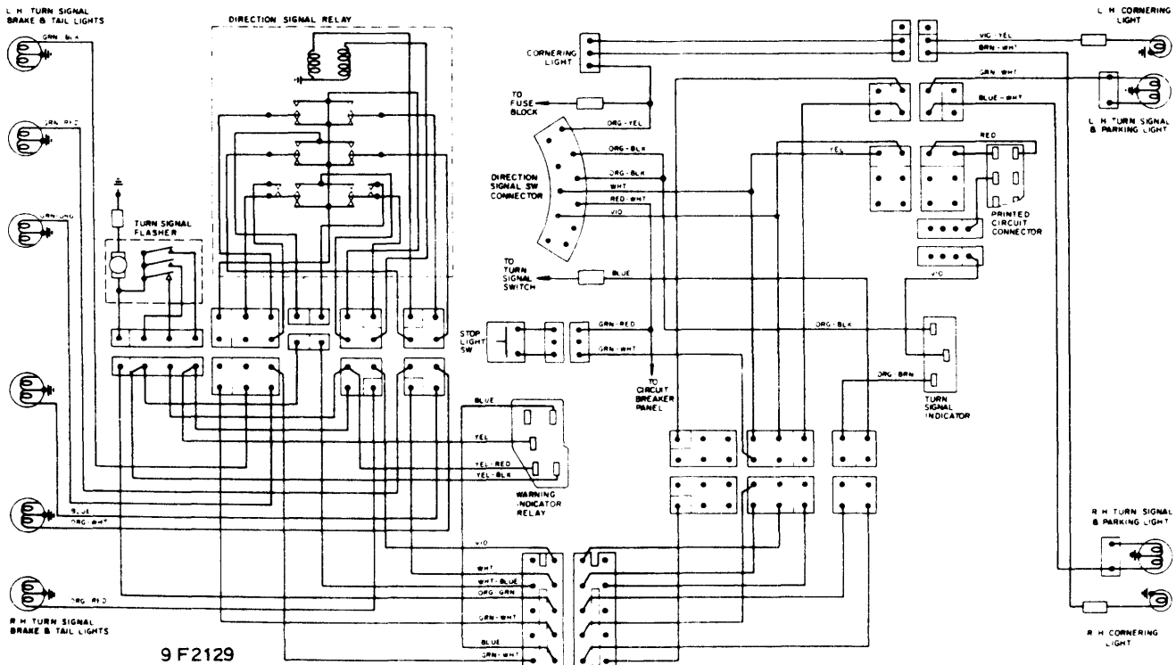
1969 THUNDERBIRD SEQUENTIAL DIRECTION SIGNALS (FIRST TYPE-MECHANICAL FLASHER UNIT)
