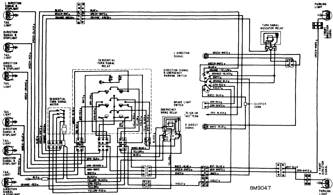
1968 COUGAR SEQUENTIAL DIRECTION SIGNALS
