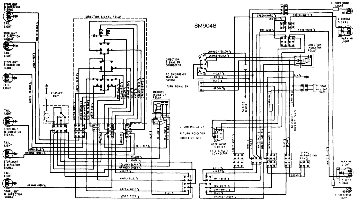
1968 THUNDERBIRD SEQUENTIAL DIRECTION SIGNALS
