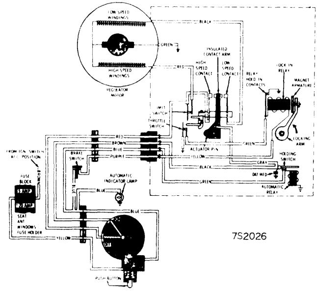
1967-68 TORONADO CRUISE CONTROL
