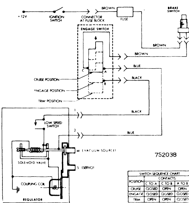
1967 PONTIAC CRUISE CONTROL
