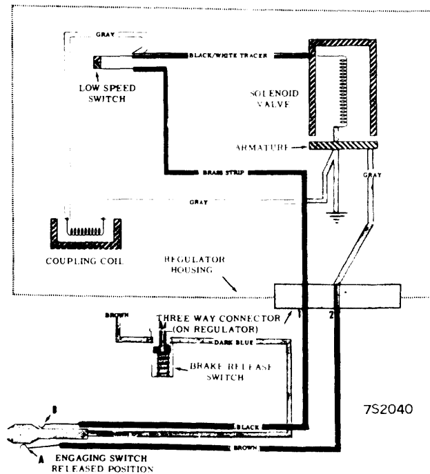
1967 OLDSMOBILE F-85 CRUISE CONTROL
