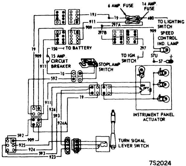
1967 LINCOLN CONTINENTAL SPEED CONTROL DIAGRAM
