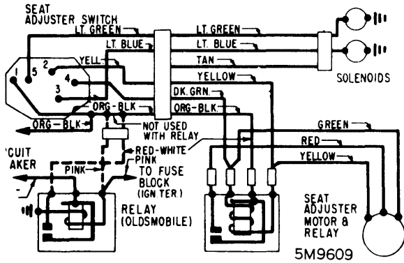
1965-67 GENERAL MOTORS 4-WAY (SWITCH IN ARM REST)
