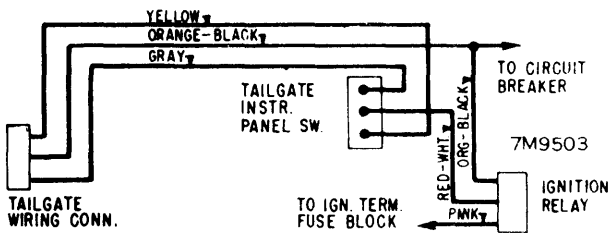
1967 CHEVELLE TAILGATE (W/O SIDE WINDOWS)
