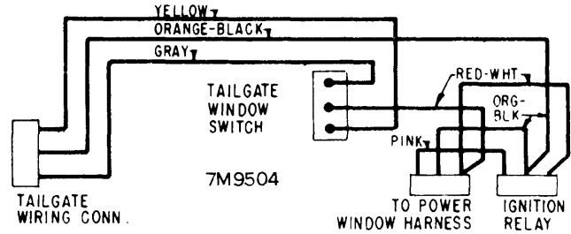
1967 CHEVELLE TAILGATE (WITH SIDE WINDOWS)
