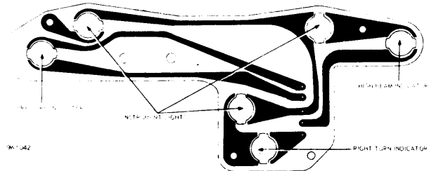
1966-67 BELVEDERE & SATELLITE (RIGHT SIDE)
