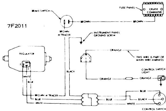
1966-67 AMERICAN MOTORS CRUISE COMMAND DIAGRAM
