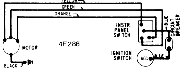
1964-66 RAMBLER TAILGATE (VERTICALLY HINGED)
