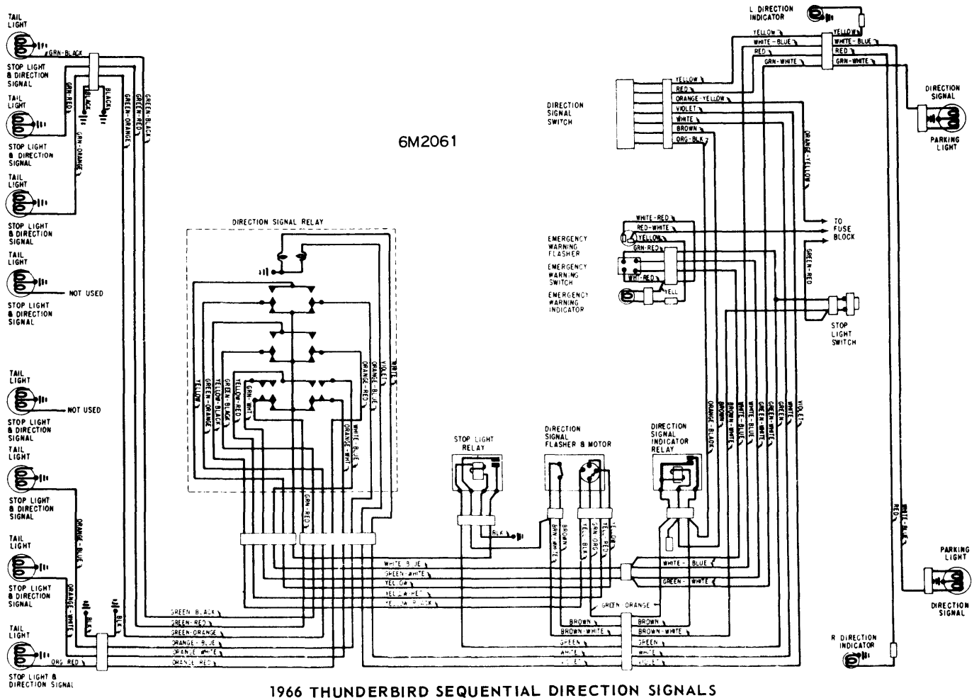
1966 THUNDERBIRD SEQUENTIAL DIRECTION SIGNALS
