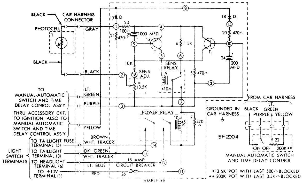
1965-66 CADILLAC TWILIGHT SENTINEL
