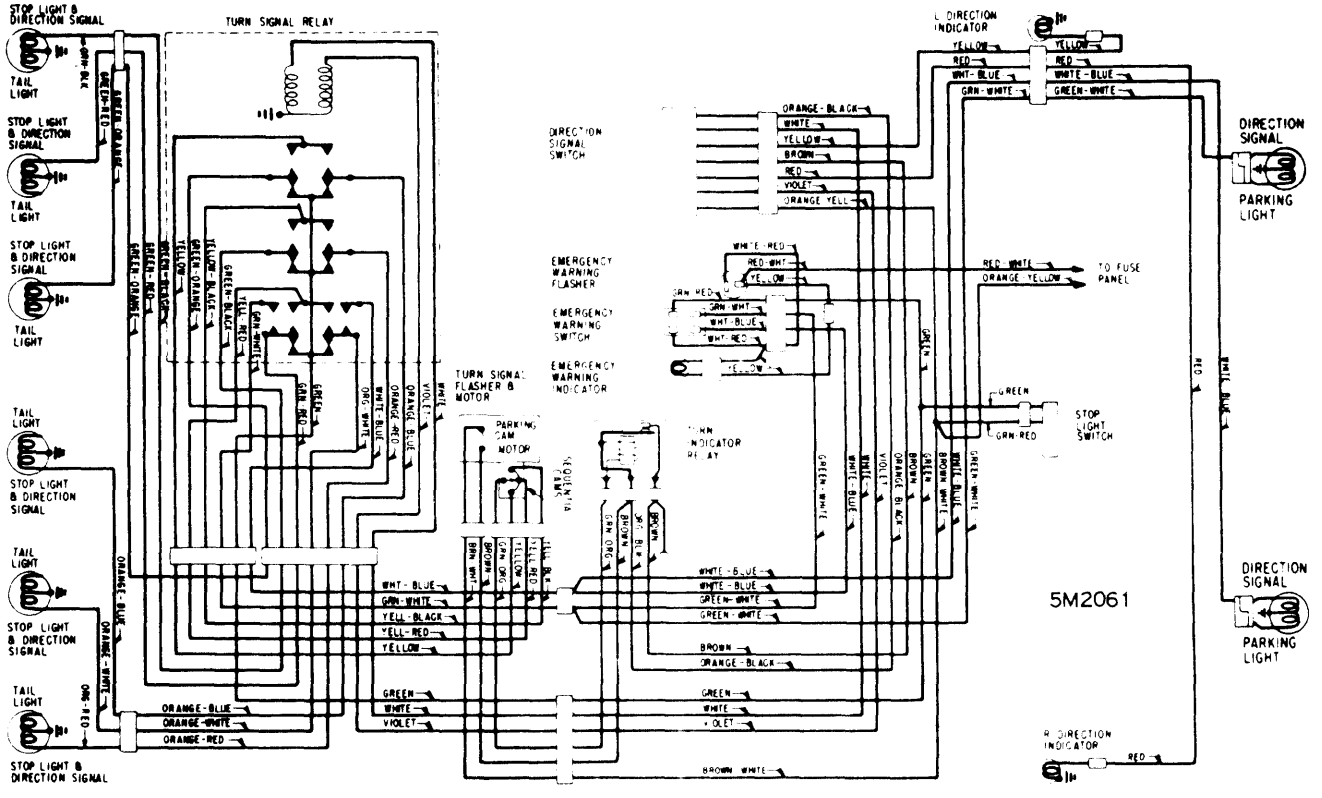
1965 THUNDERBIRD SEQUENTIAL DIRECTION SIGNALS
