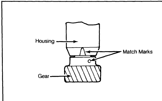
Fig. 5: Installing Driven Gear on Distributor Shaft
