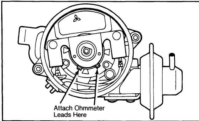
Fig. 2: Checking Pick-Up Coil Resistance
