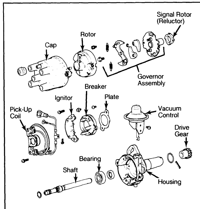
Fig. 7: Exploded View of Chrysler Corp. Distributor
