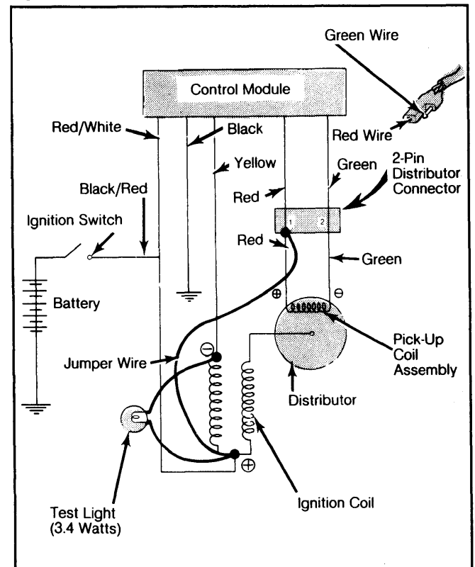
Fig. 4: Checking Courier 2300 cc Ignition Control Module
