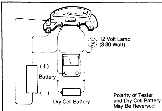
Fig. 3: Checking Chrysler Corp. Ignitor with Battery and Test Lamp
