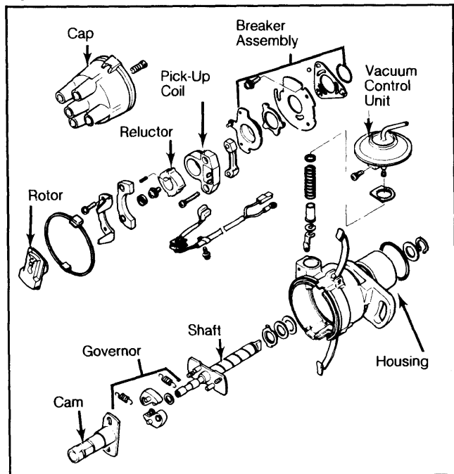
Fig. 6: Exploded View of Mazda Distributor
