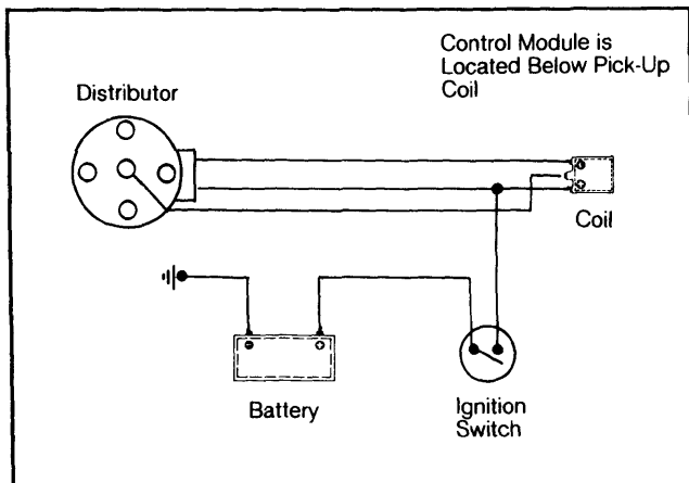
Fig. 1: Wiring Schematic of Mitsubishi Electronic Ignition System With Internal Control Module
