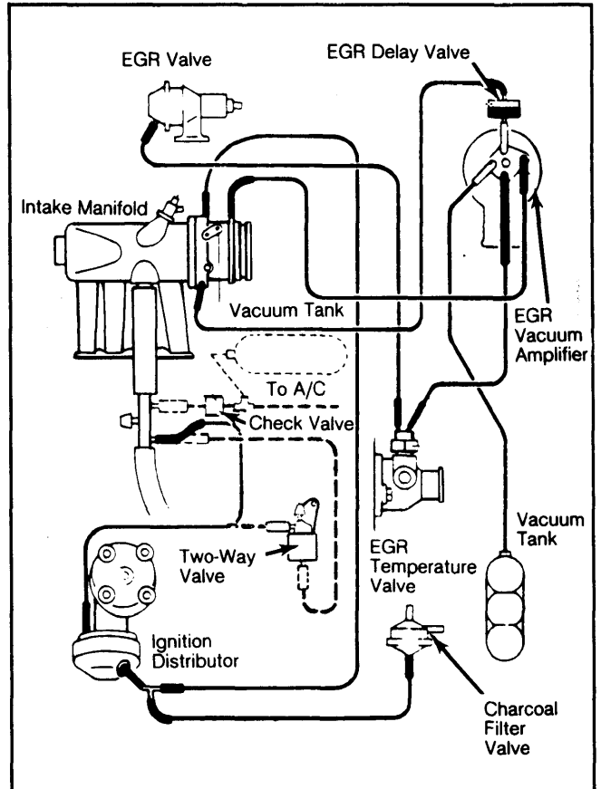
Fig. 2: Volkswagen Vacuum Diagram (Rabbit Pickup)
