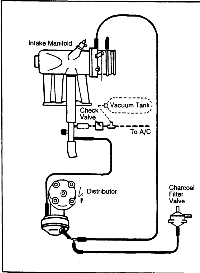
Fig. 1: Volkswagen Vacuum Diagram (Jetta, Rabbit & Scirocco)
