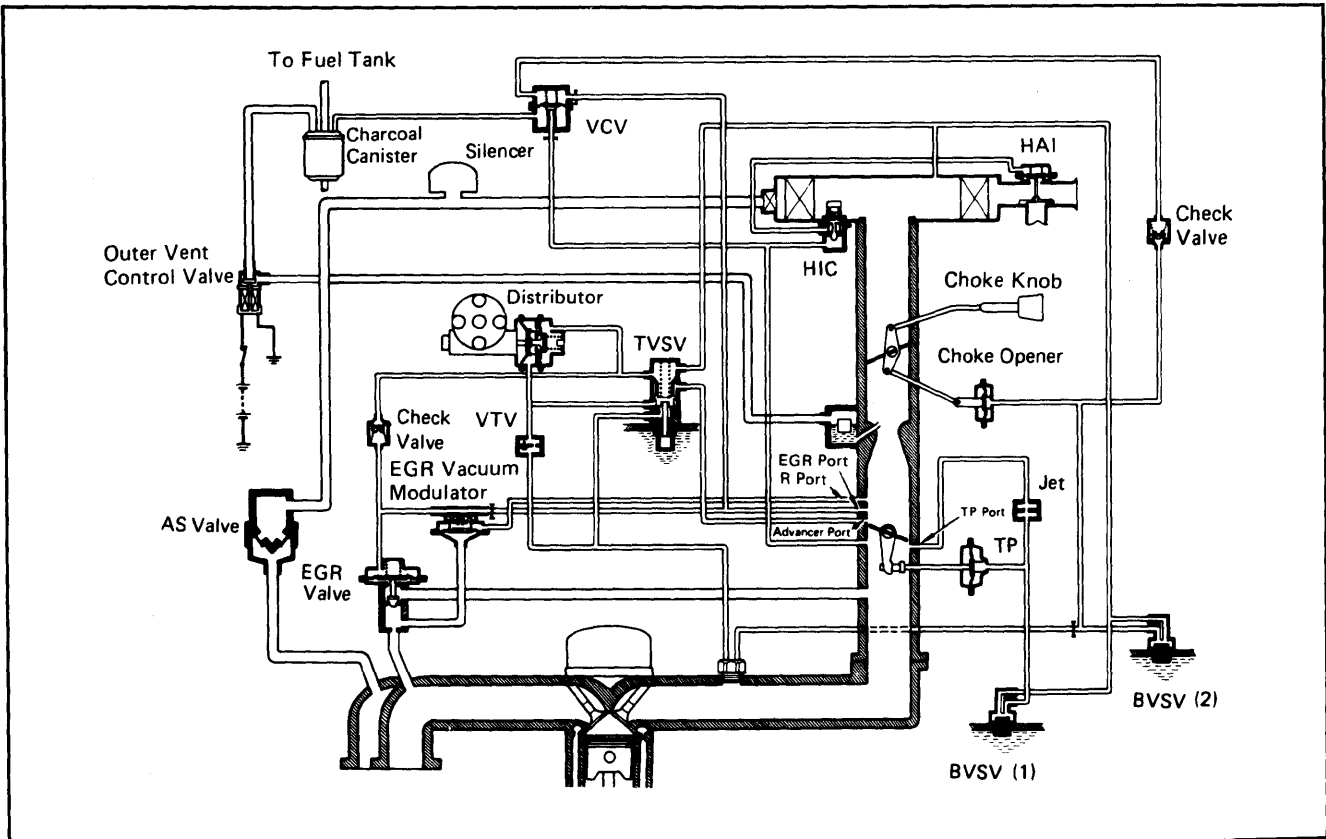
Fig. 10: Starlet without High Altitude Compensation (HAC) System
