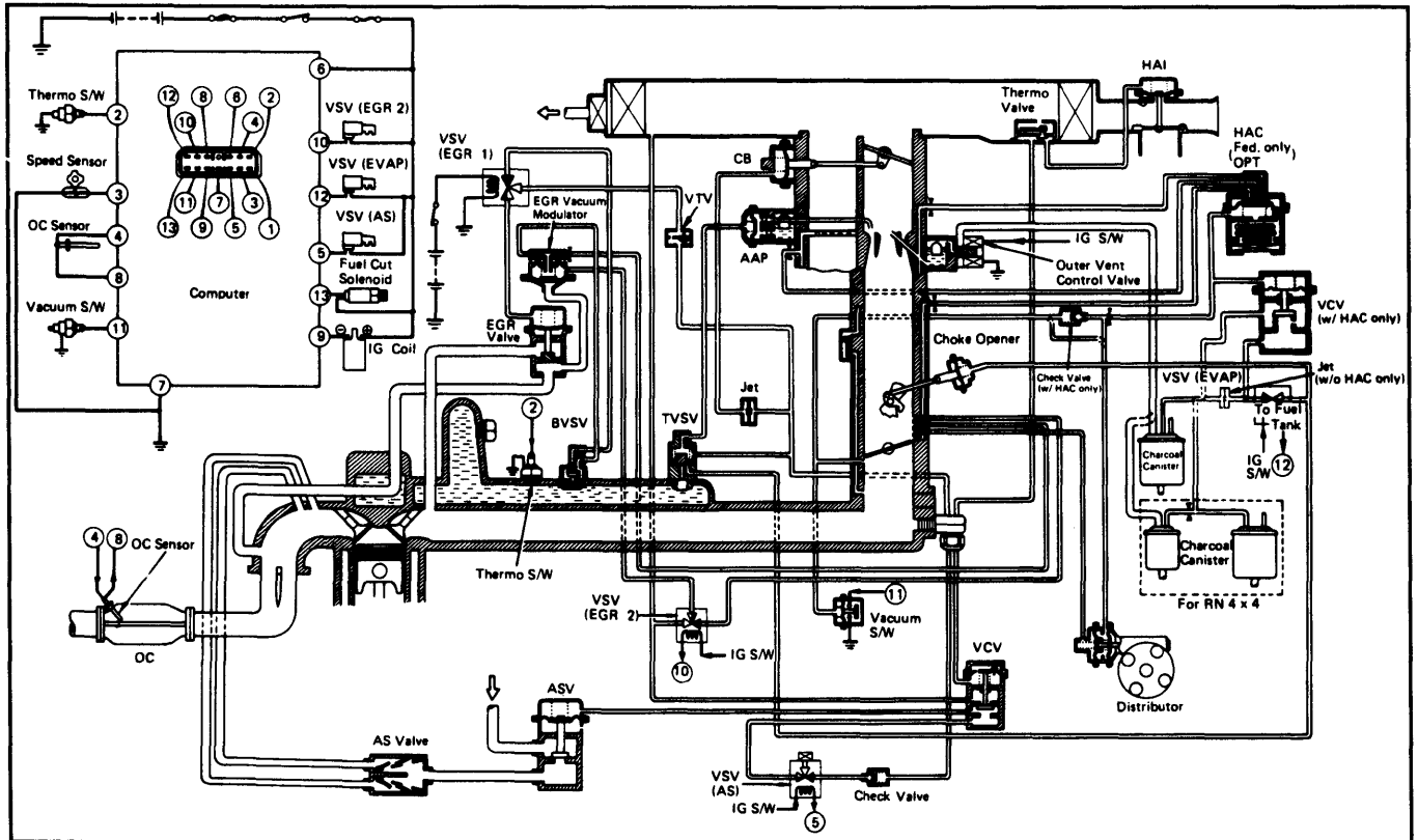
Fig. 8: Pickup Federal Auto Trans.
