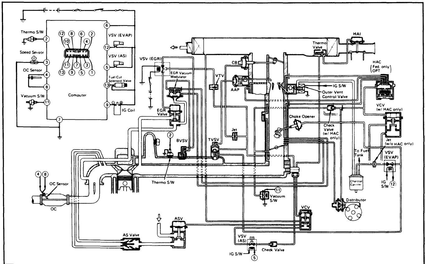
Fig. 8: Pickup Federal Auto Trans.
