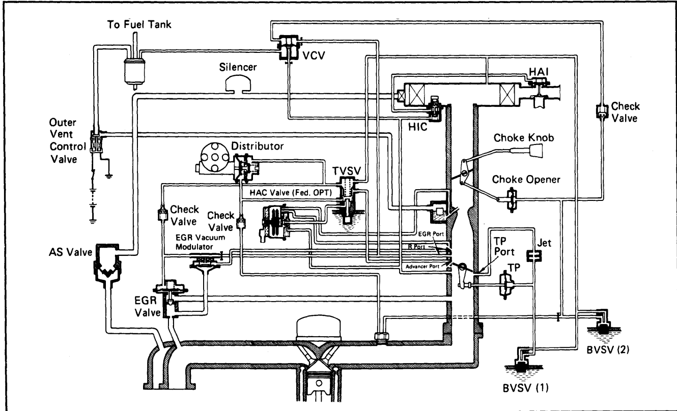
Fig. 9: Starlet with High Altitude Compensation (HAC) System
