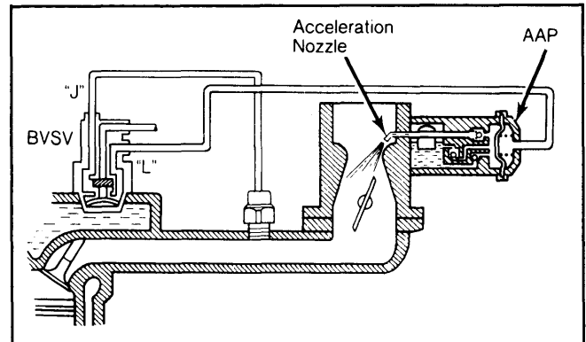
Fig. 2: Celica & Pickup AAP System
