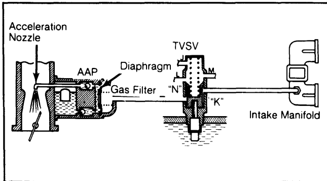
Fig. 1: Corolla AAP System
